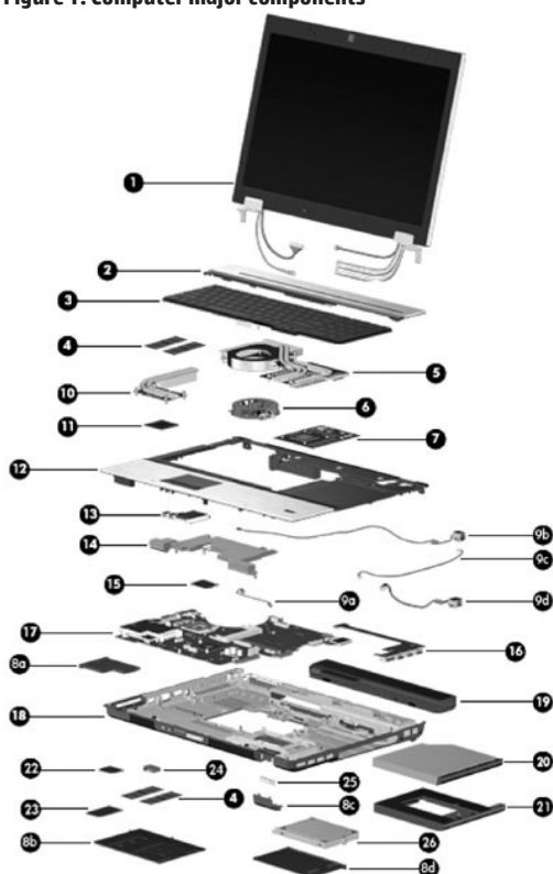
Figure 1: Computer major components
