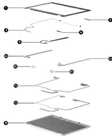
Figure 3: Display components
